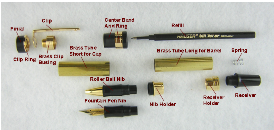
Parts Diagram for the El Grande Roller Ball and Fountain Pen
