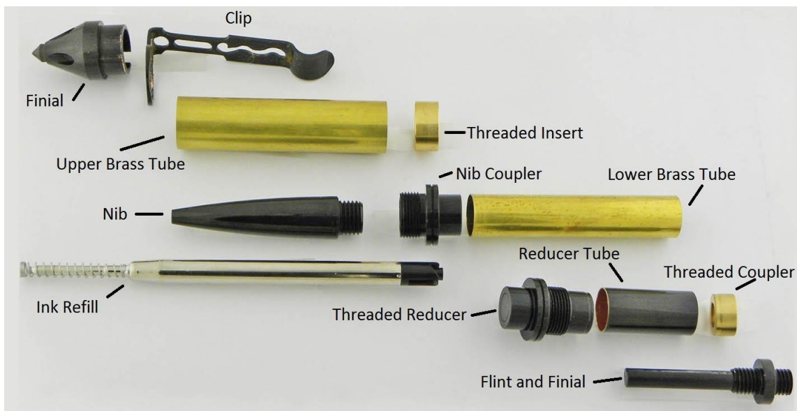
Parts Diagram for the Survival Ballpoint Pen
