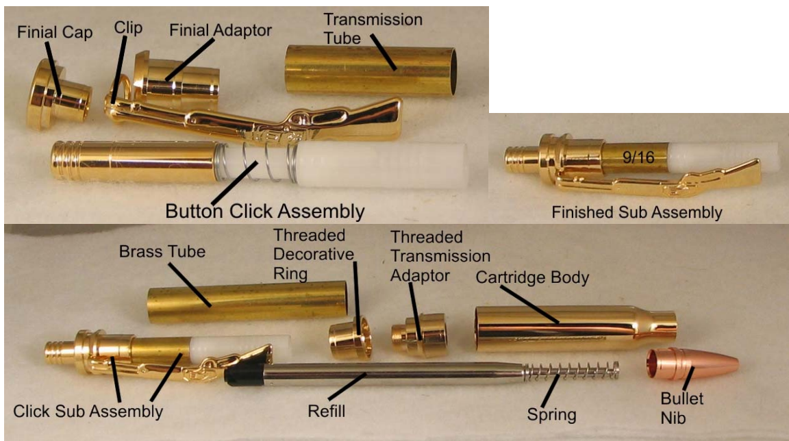
Parts Diagram
