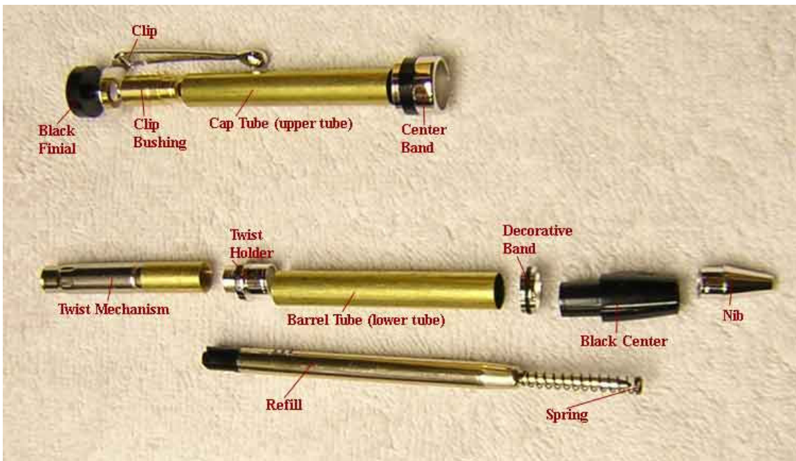
Pen Parts Diagram
