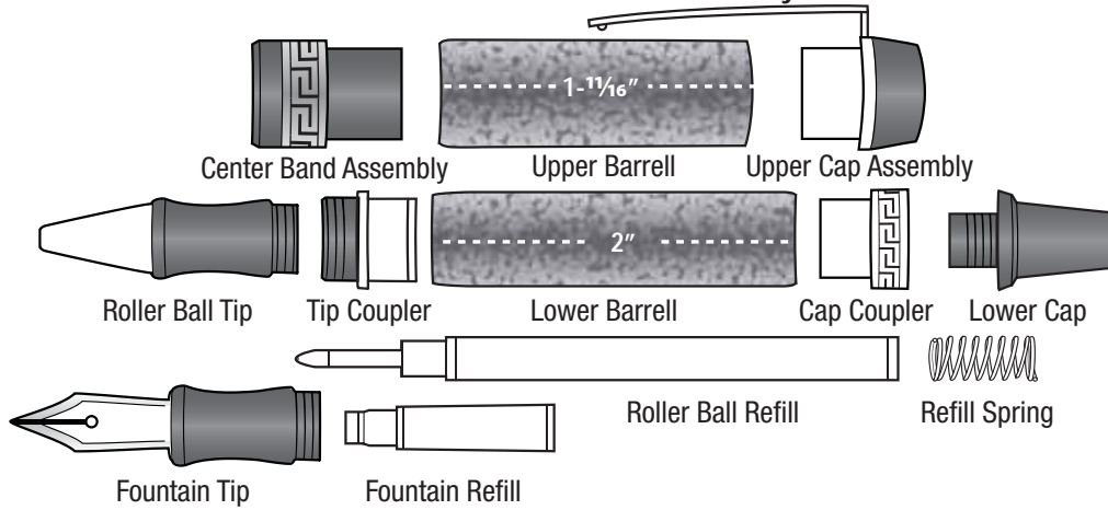
DIAGRAM C • Pen Assembly
